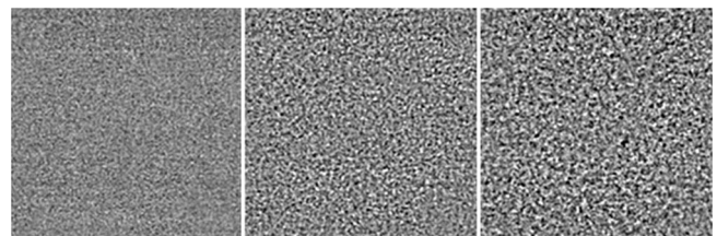
FIG. 2. Images obtained by subtracting two microscopy images that are taken at time intervals of \Delta t = 0.01, 0.1, and 1 s (from left to right). The subtraction removes efficiently the stray signal and isolates the contribution due to the particles. The average size of the speckles gives an estimate of the microscope resolution. The contrast in the images increases with \Delta t .
